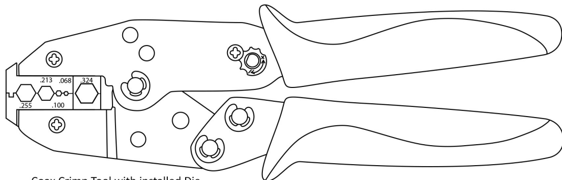
Coax Crimp Tool with installed Die
