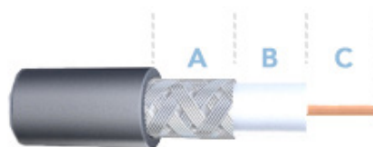
Recommended Cable Strip Dimensions
